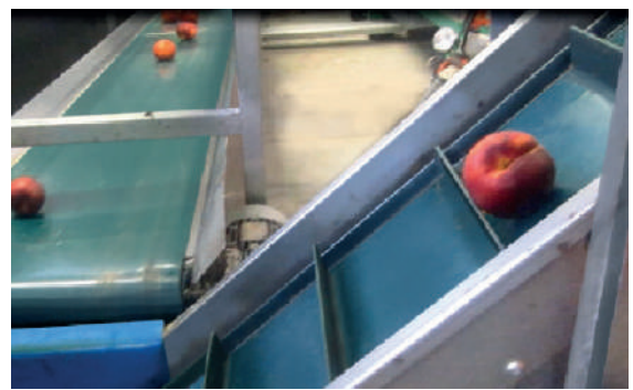
FEBOR 14CF GR EU with transverse cleats and longitudinally cut profiles.
